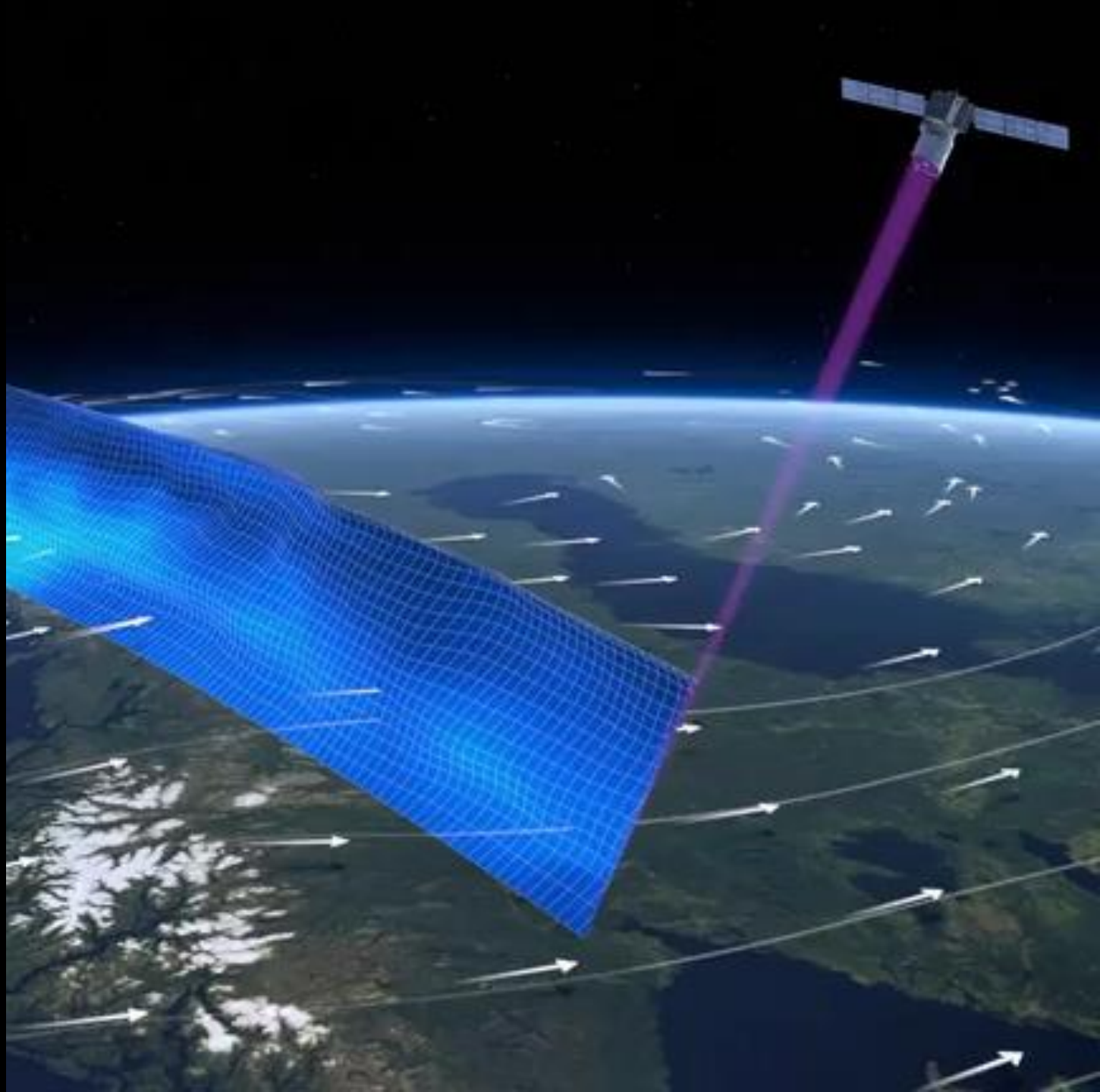
First global maps of wind Aeolus-1, 2016 Source: ESA
